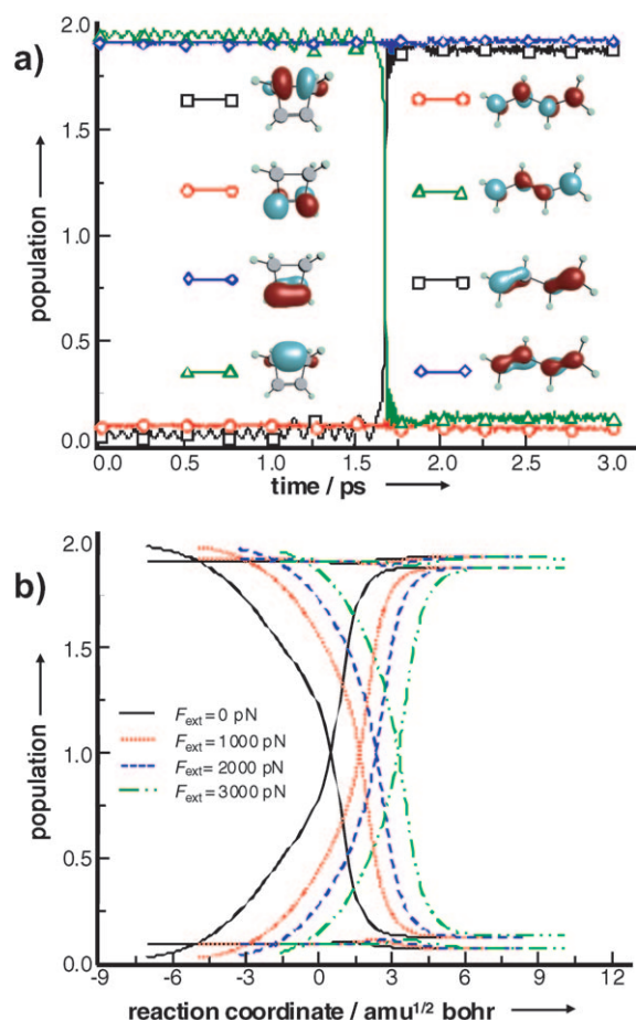
Figure 1. a) Populations of the natural orbitals comprising the active space during the MD simulation with F_{\text{ext}} = 2800 pN. The orbitals in the reactants and products are shown at the left and right, respectively, and different colored curves denote correlated orbitals. The orbitals are plotted at contour values of 0.1 au, and colors indicate different phases of the wavefunction. The orbitals are arranged from bottom to top in increasing energy. b) Populations of the natural orbitals comprising the active space along the IRCs. The orbitals monitored are analogous to those shown in (a). The transition state is located at 0 \text{ amu}^{1/2} \text{ bohr} . Four curves are shown for each F_{\text{ext}} .
